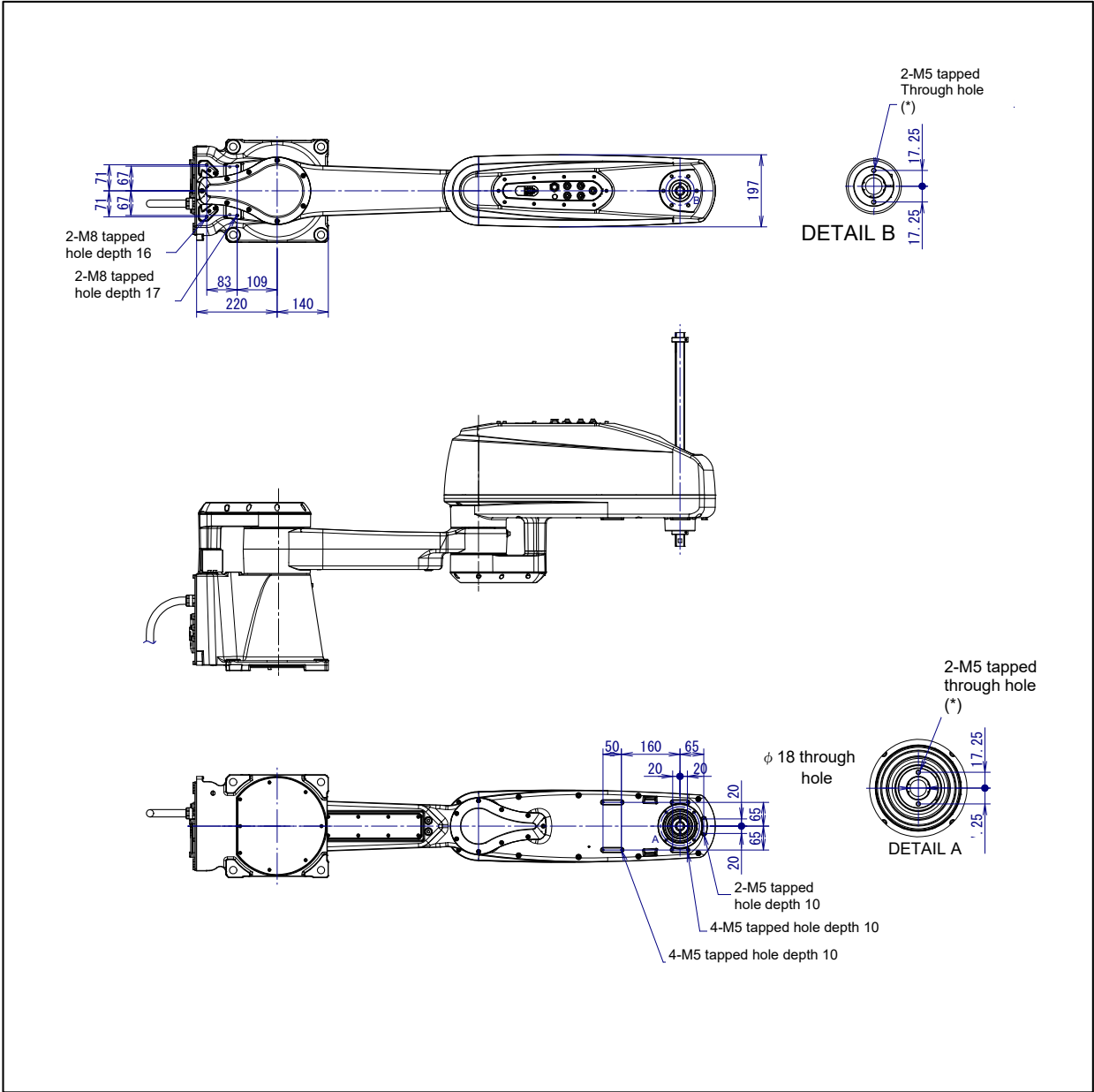
Fig. 4.2 (c) Equipment mounting faces (SR-20iA)
