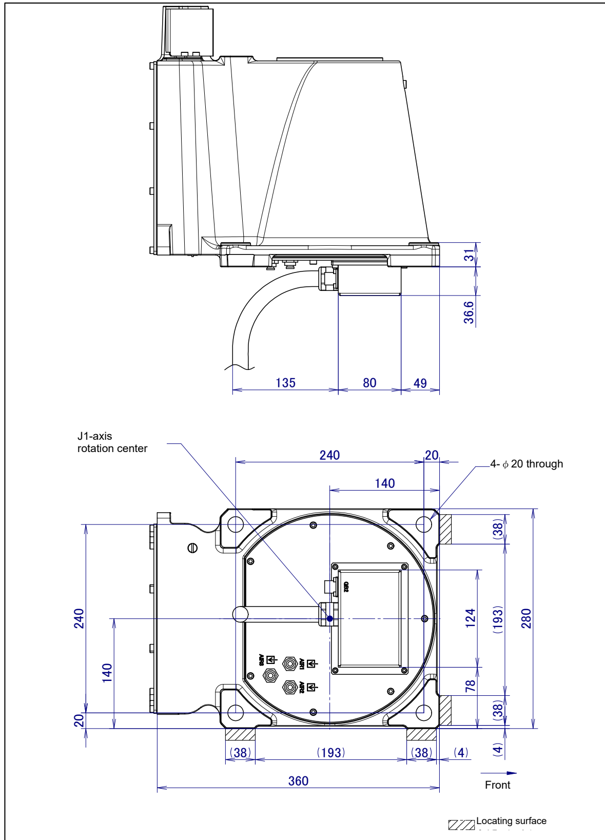
Fig. 1.2 (b) Dimensions of the robot base (bottom side connector panel)
