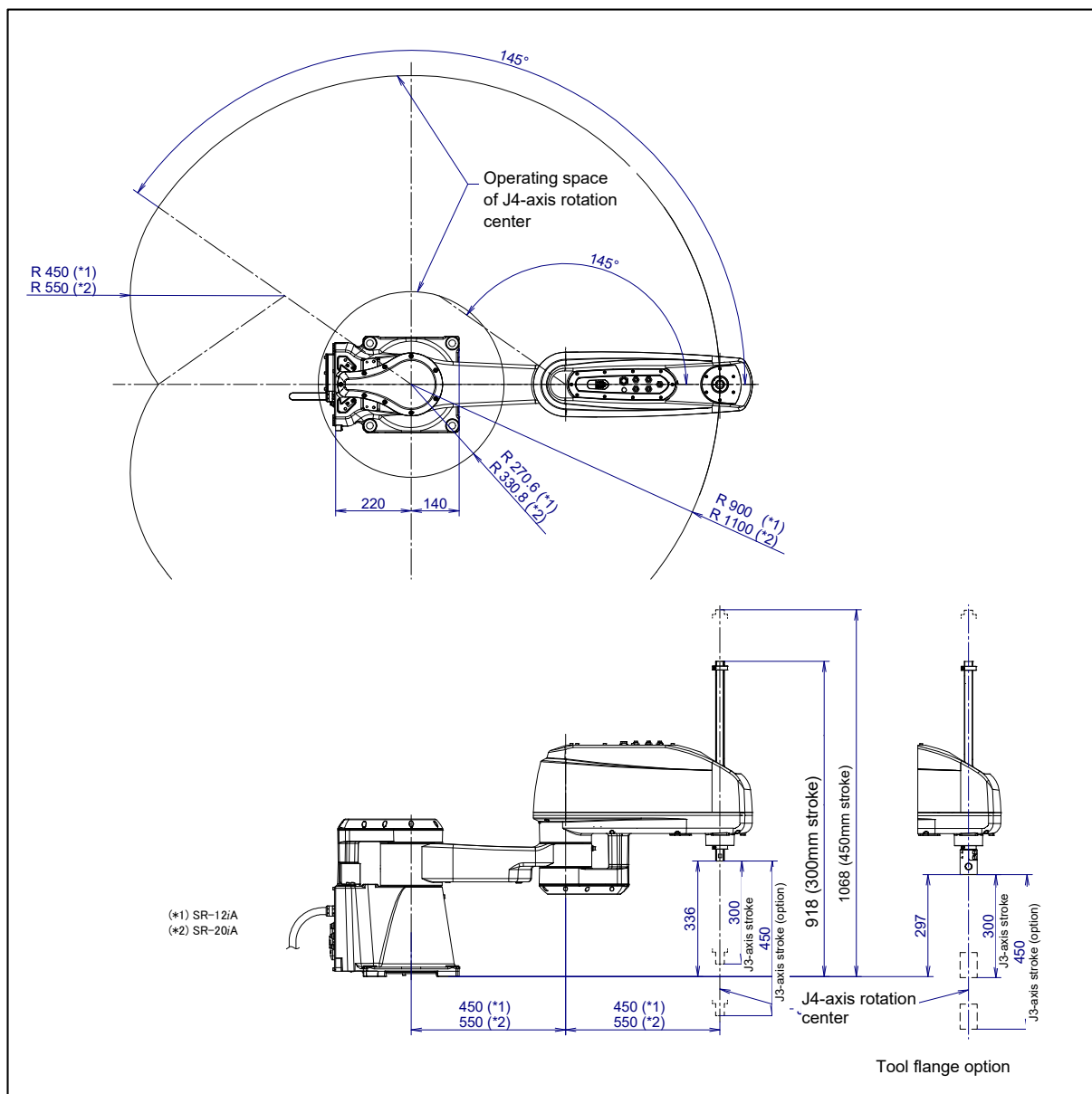
Fig. 3.2 (a) Operating space
