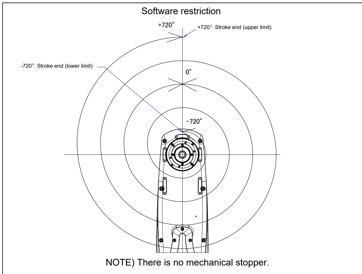
Fig. 3.3 (f) J4-axis motion limit
