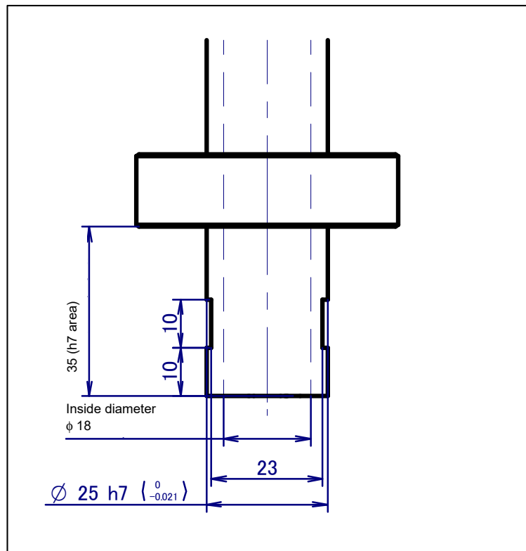
Fig. 4.1 (a) Surface for installing the end effector
