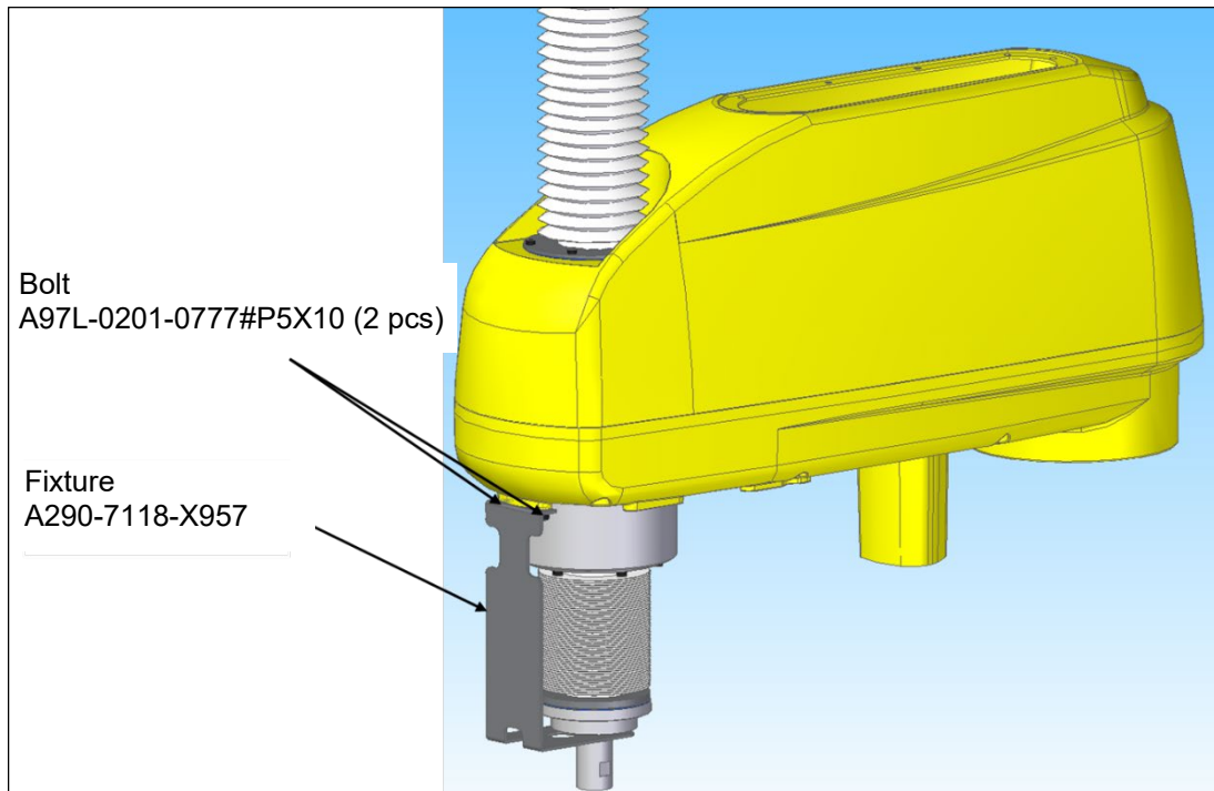
Fig. 8.3.1 (a) Fixture installation
