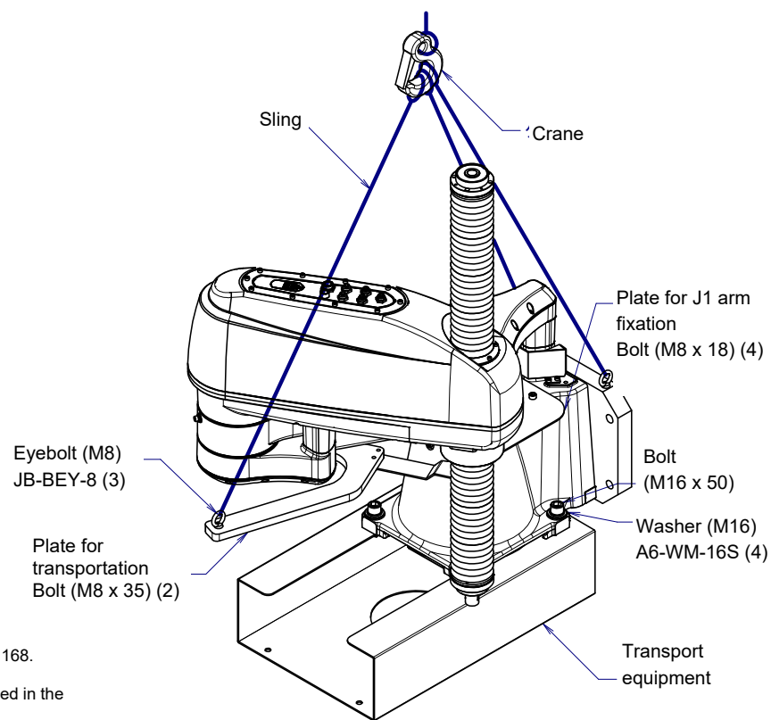
Fig. 1.1 (b) Transportation using a crane (wall mount)
