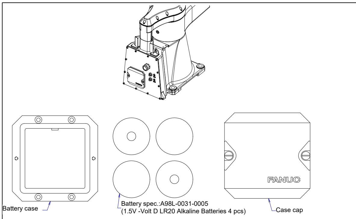
Fig. 7.3.1 (a) Replacing the battery (if built-in batteries are specified)
