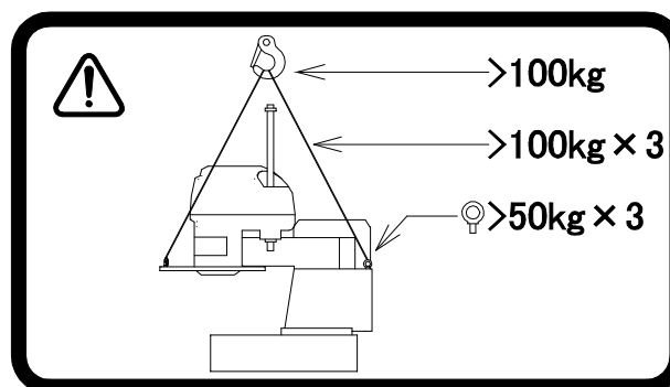
Fig. 5 (a) Transportation label
