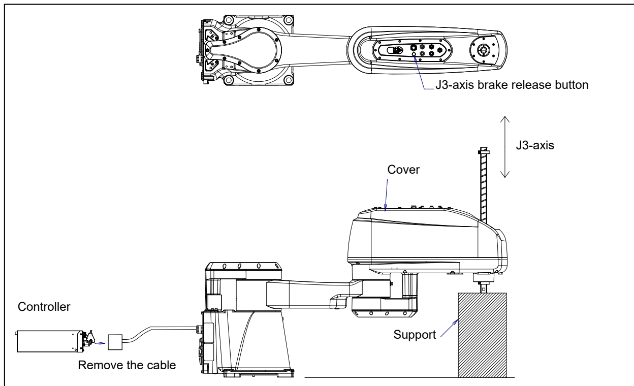
Fig. 3 (a) J3-axis brake release button
