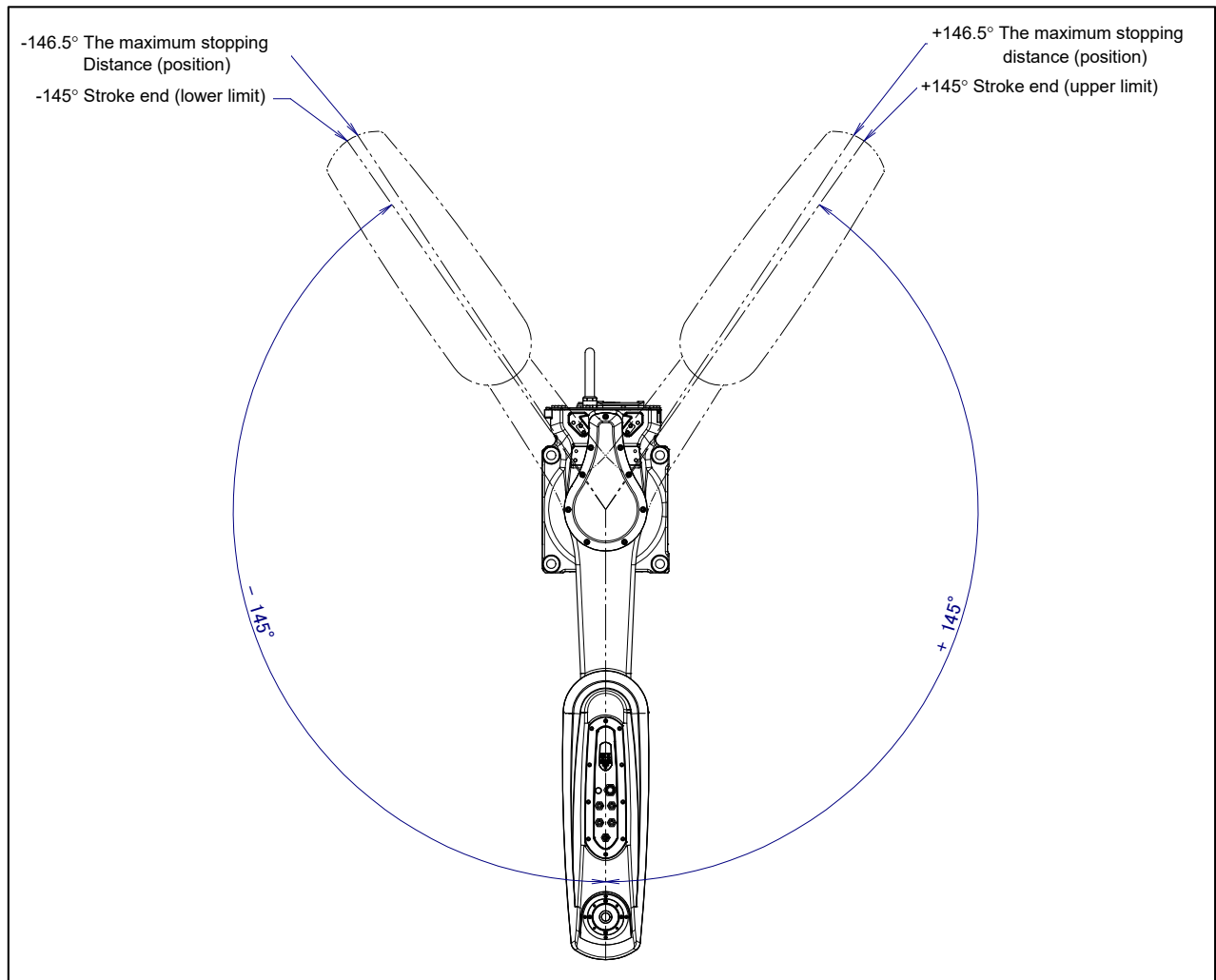
Fig. 3.3 (b) J1-axis motion limit
