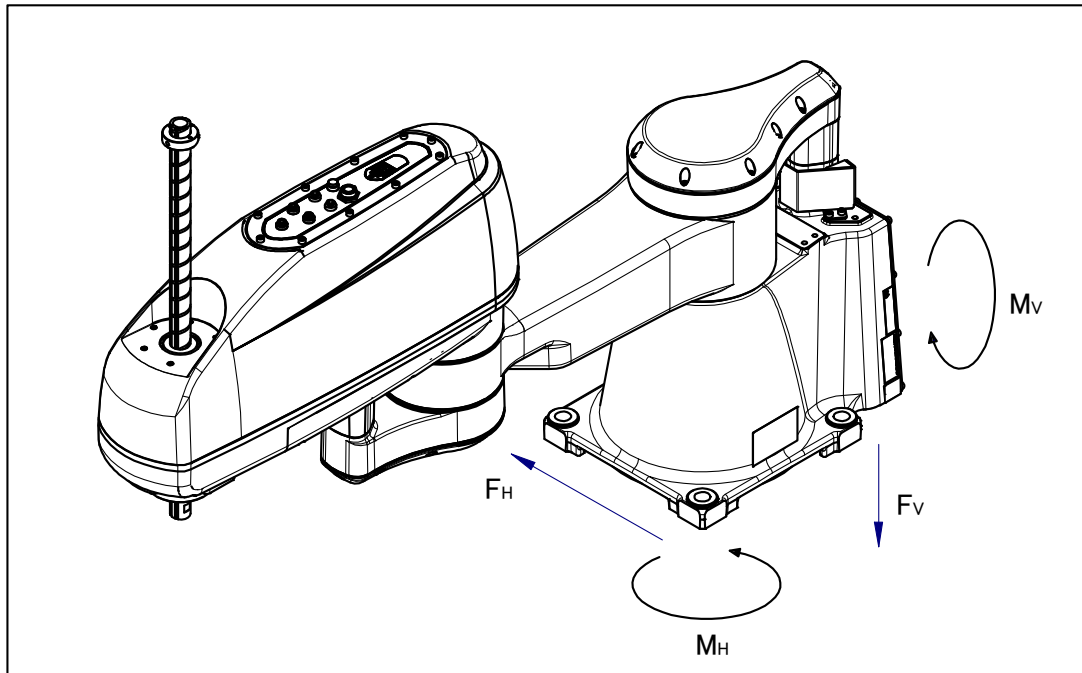
Fig. 1.2.1 (c) Force and moment that acts on J1 base
