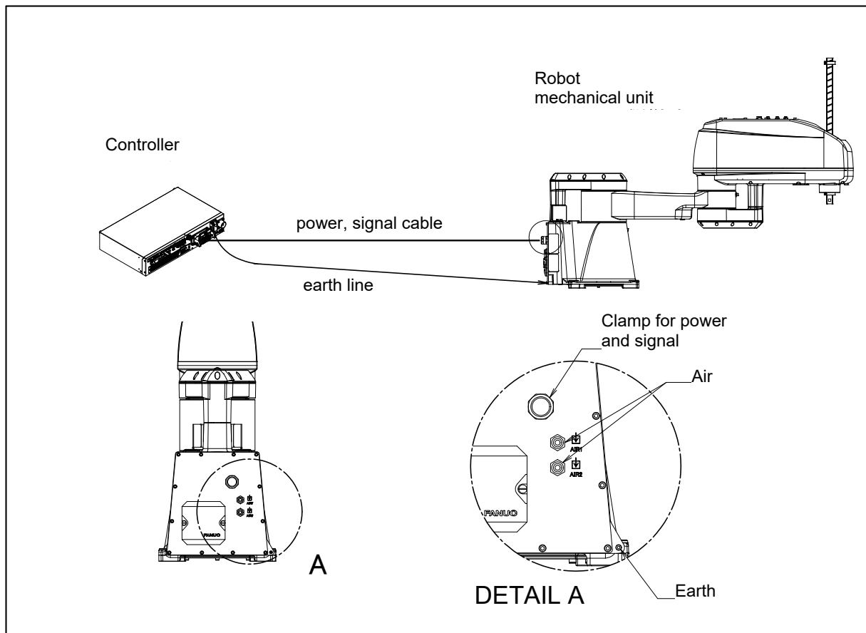
Fig. 2 (a) Cable connection (back side connector panel)
