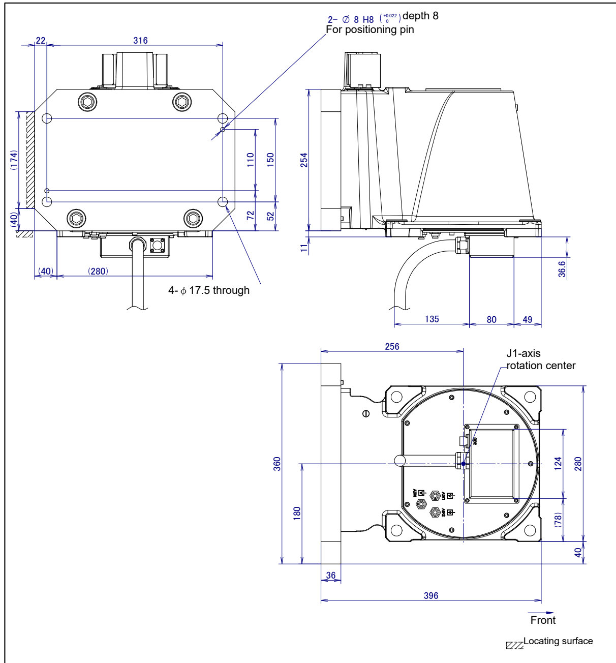
Fig. 1.2 (c) Dimensions of the robot base (wall mount specification)
