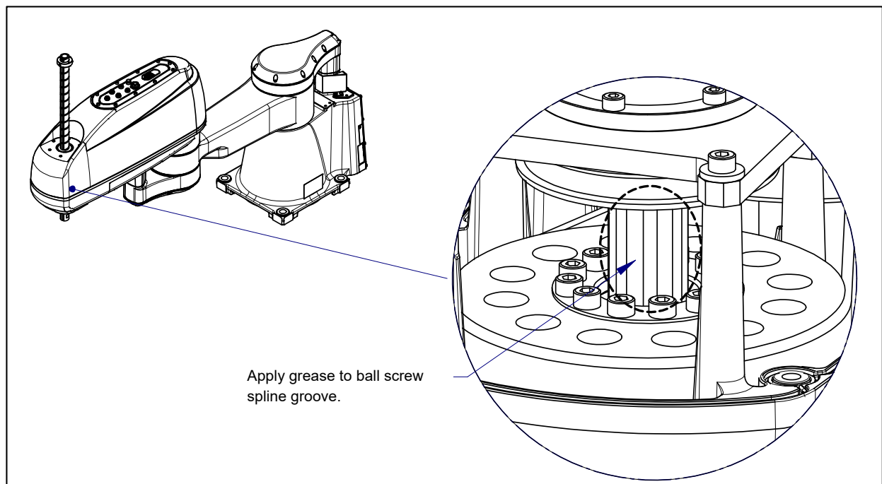
Fig. 7.3.4 (c) Applying grease of ball screw spline
