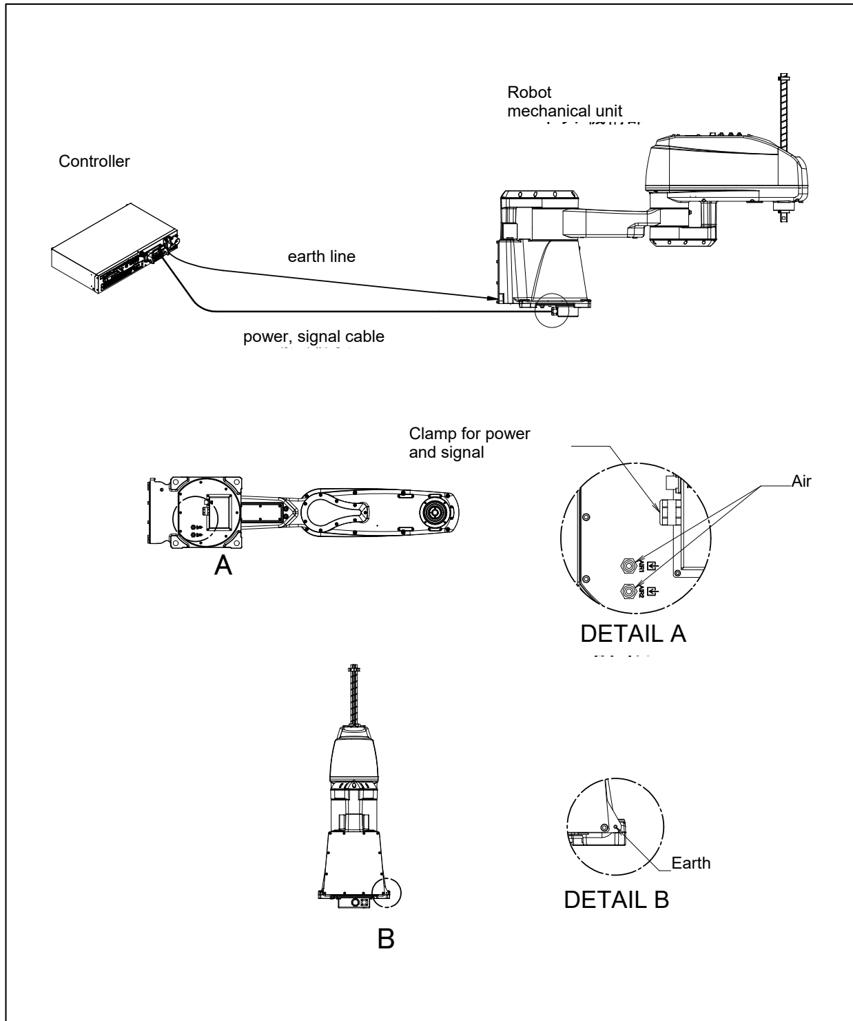
Fig. 2 (b) Cable connection (bottom side connector panel)
