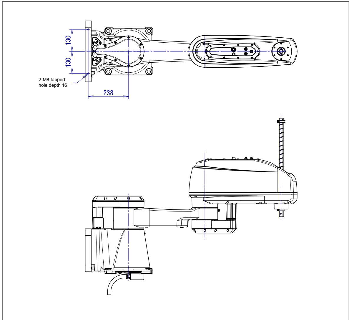
Fig. 4.2 (d) Equipment mounting faces (SR-12iA, SR-20iA) (wall mount)
