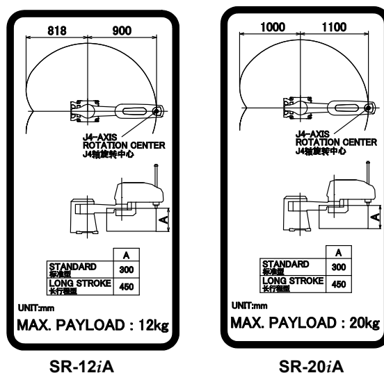
Fig. 5 (b) Operating space and payload label
