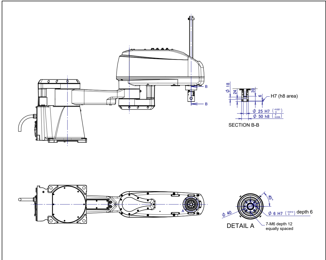
Fig. 4.2 (b) Equipment mounting faces (SR-12iA, SR-20iA) (tool flange option)
