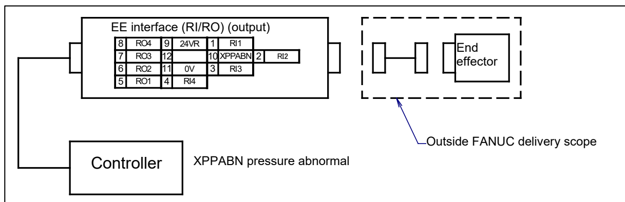
Fig. 5.2 (c) EE (RI/RO) interface (When A05B-1118-H201,H251,H301,H351 is specified)
