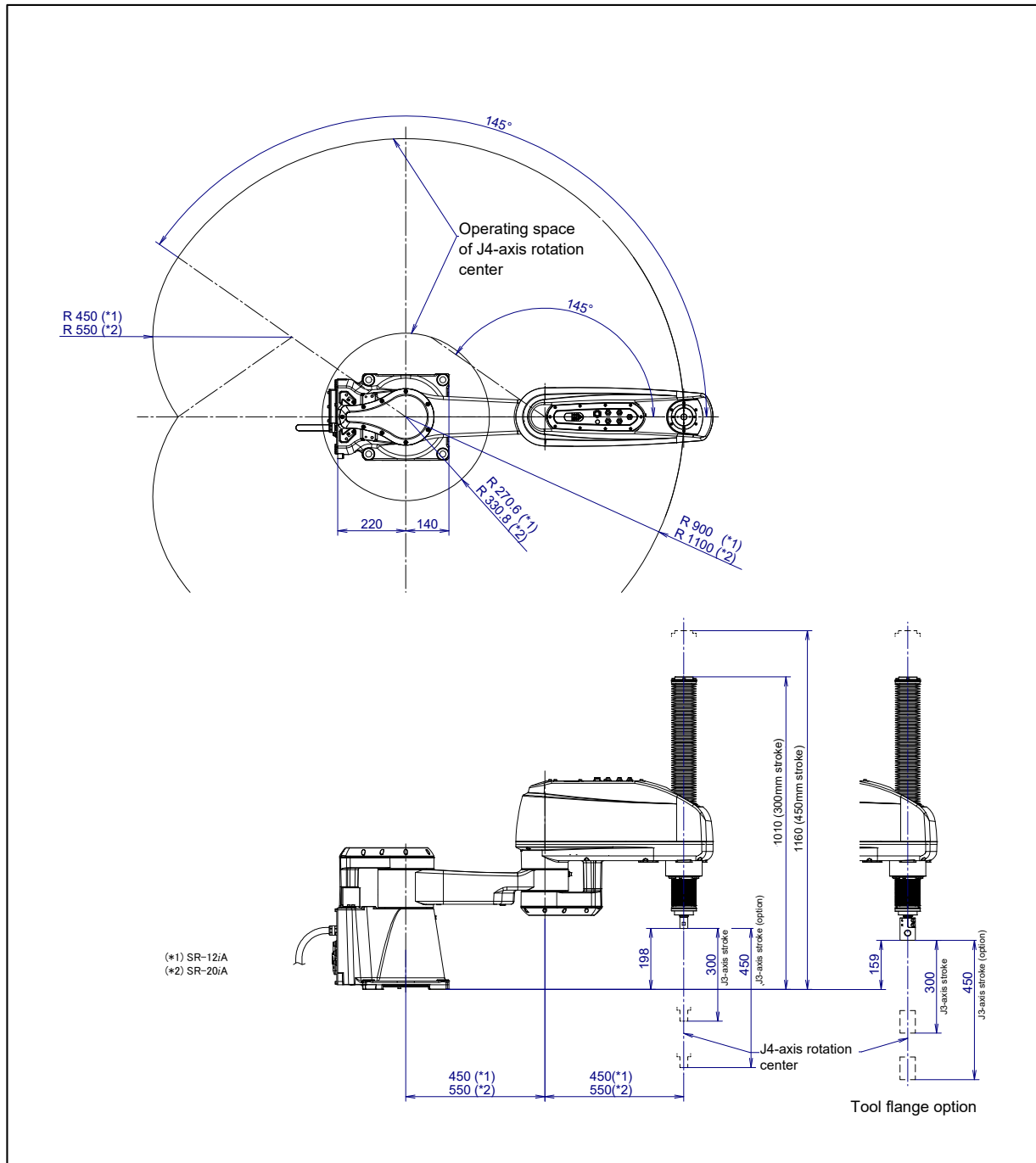
Fig. 3.2 (b) Operating space (bellows option)
