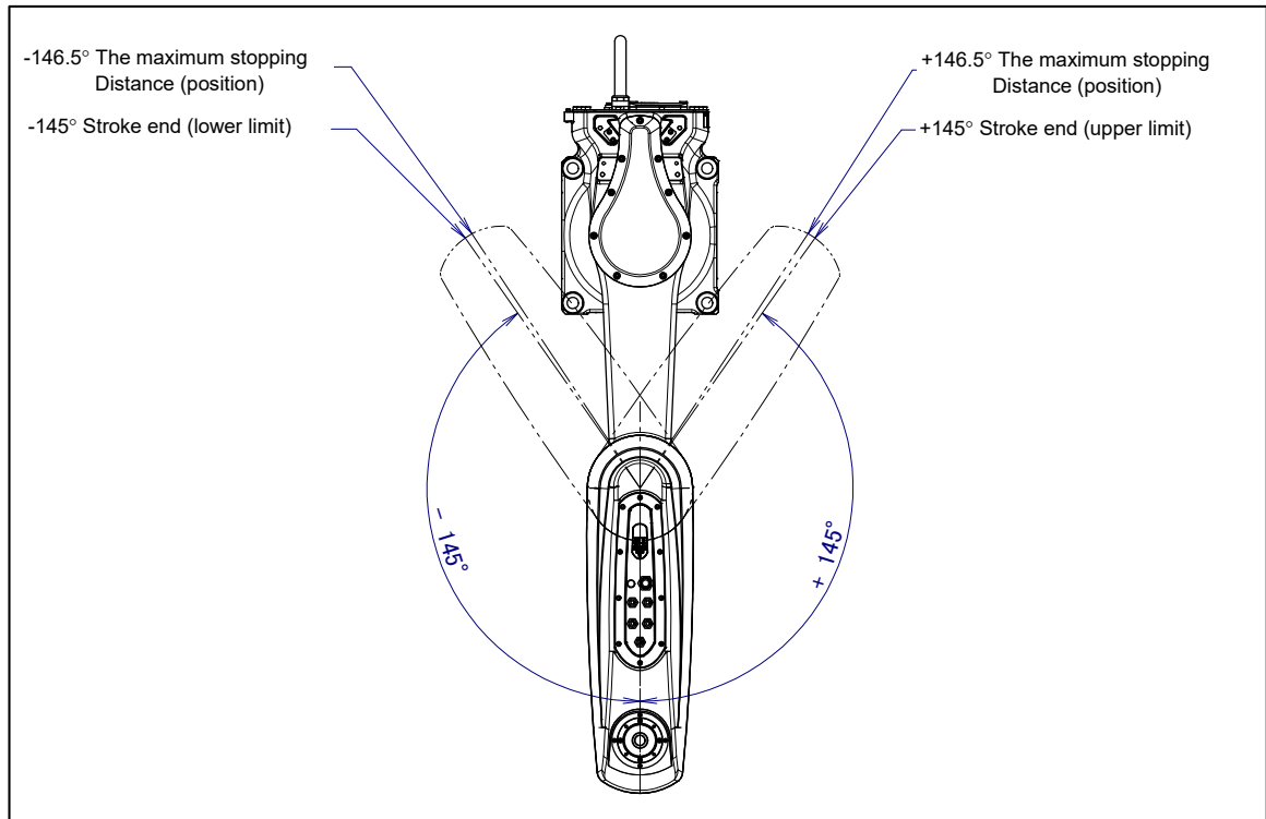
Fig. 3.3 (c) J2-axis motion limit
