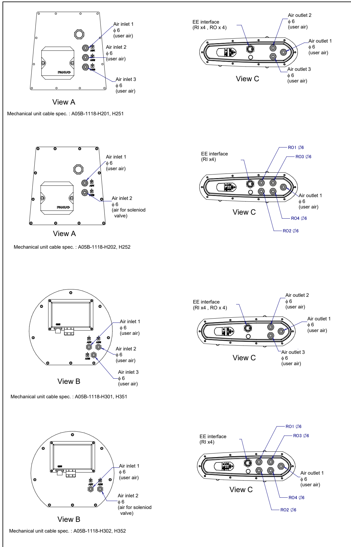
Fig. 5.2 (b) Air supply and EE (RI/RO) interface
