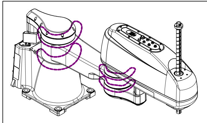
Fig. 7.2.1 (a) Check points of oil seepage
