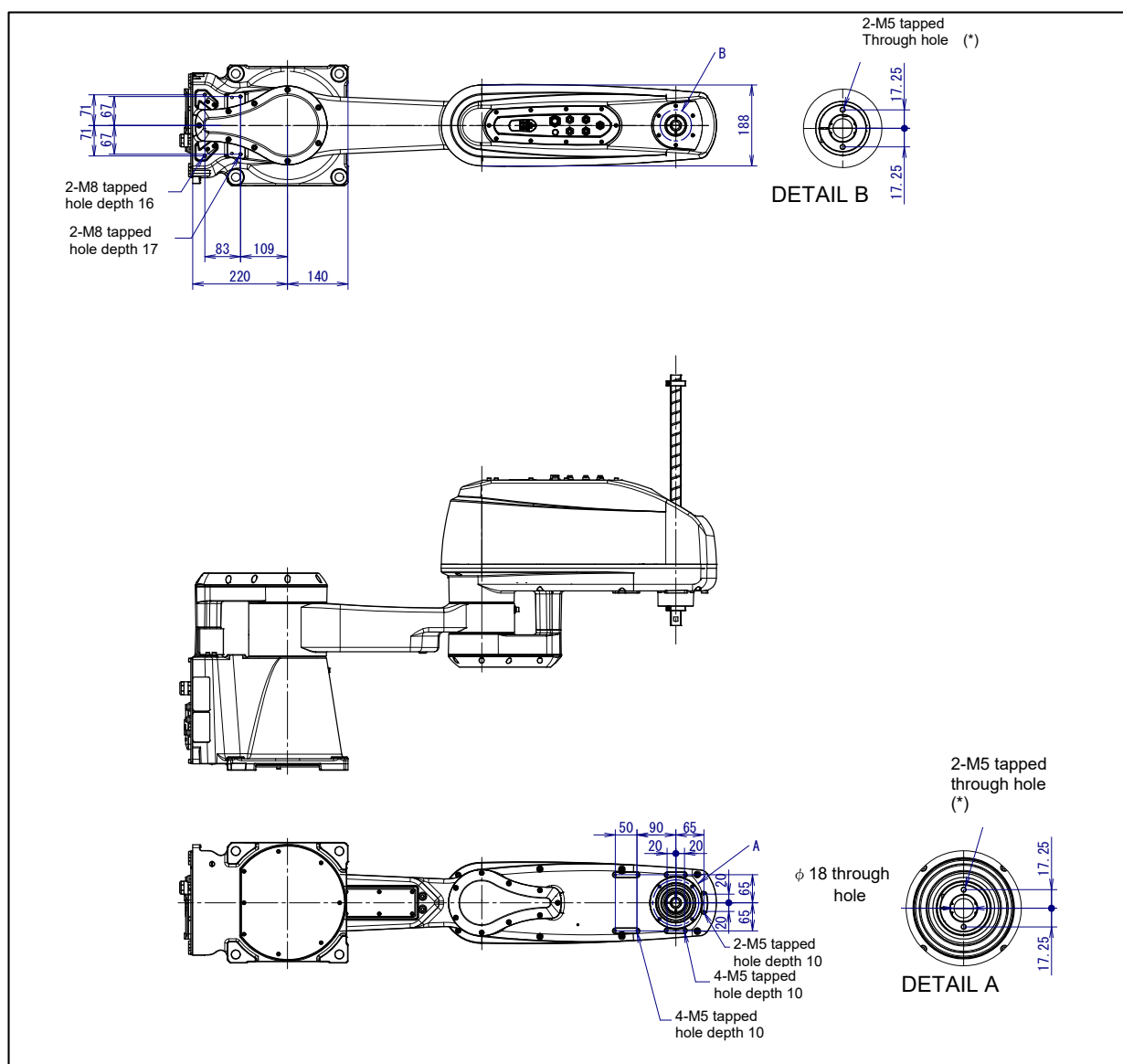
Fig. 4.2 (a) Equipment mounting faces (SR-12iA)
