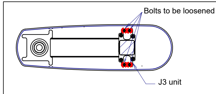
Fig. 3 (b) Bolt position to be loosened
