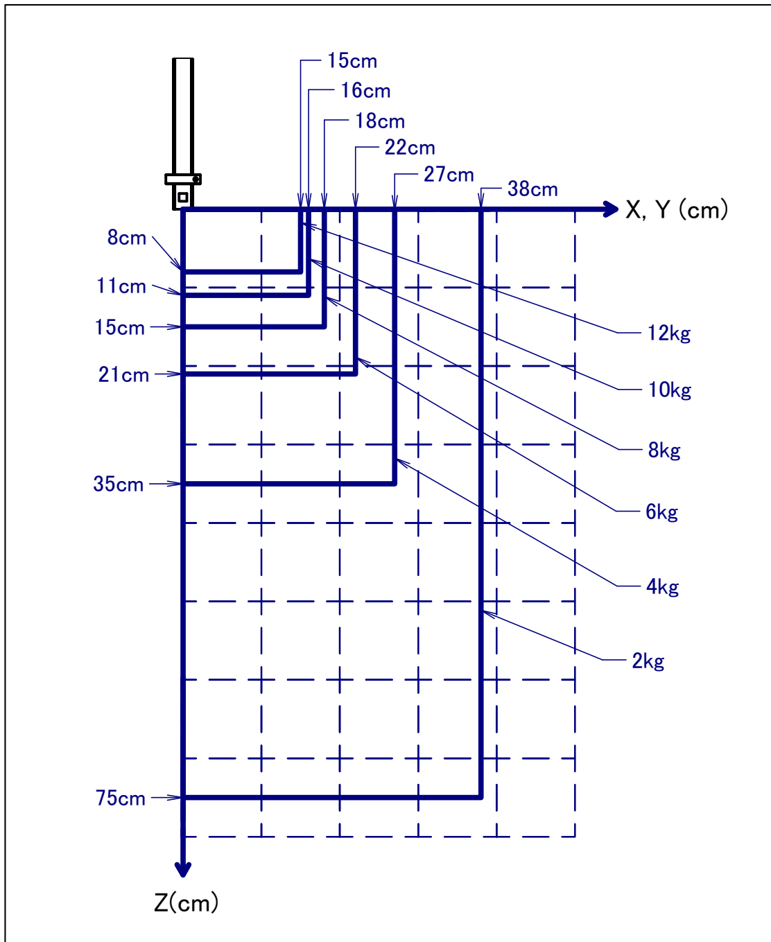
Fig. 3.4 (a) Wrist load diagram (SR-12iA)
