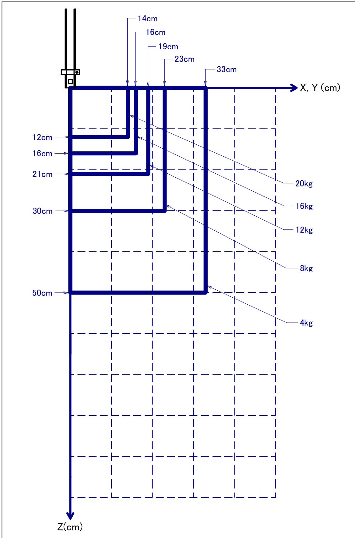
Fig. 3.4 (b) Wrist load diagram (SR-20iA)
