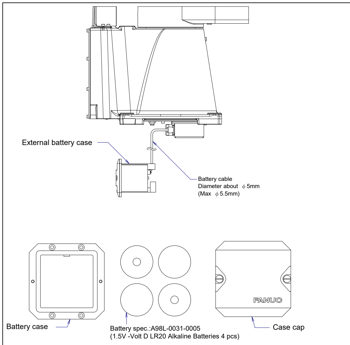
Fig. 7.3.1 (b) Replacing the battery (if external batteries are specified)
