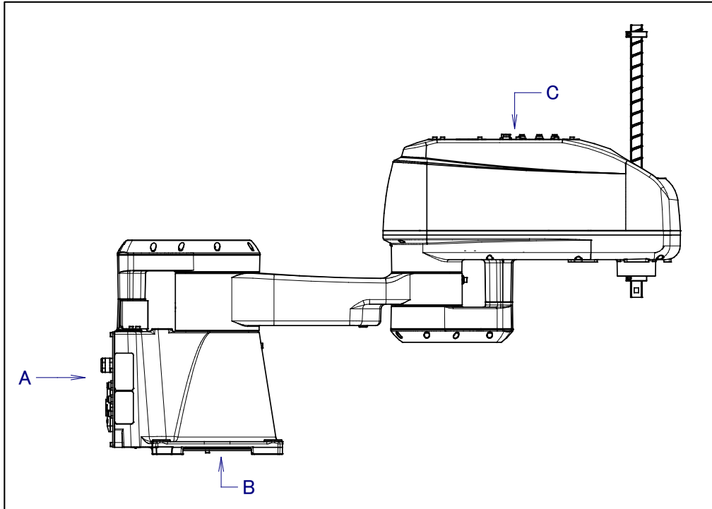
Fig. 5.2 (a) Air supply and EE (RI/RO) interface position
