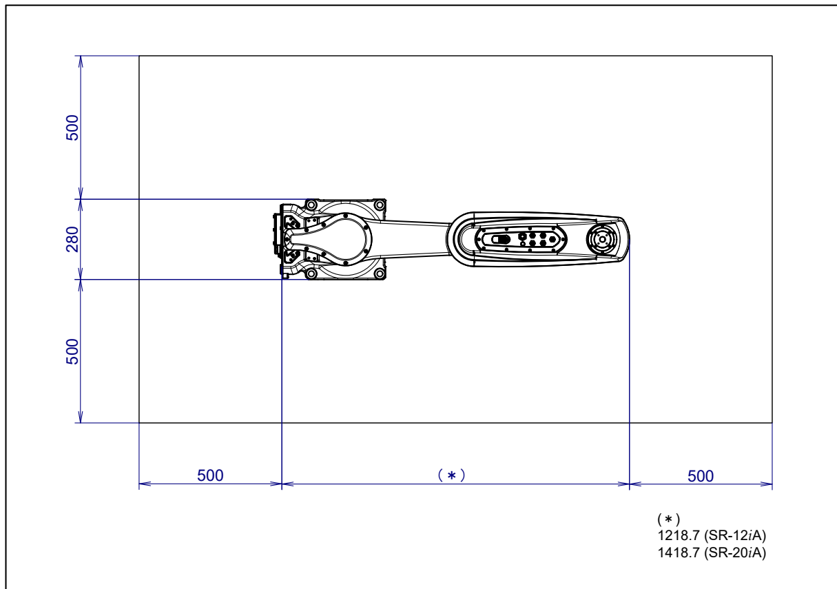
Fig. 1.3 (a) Maintenance area
