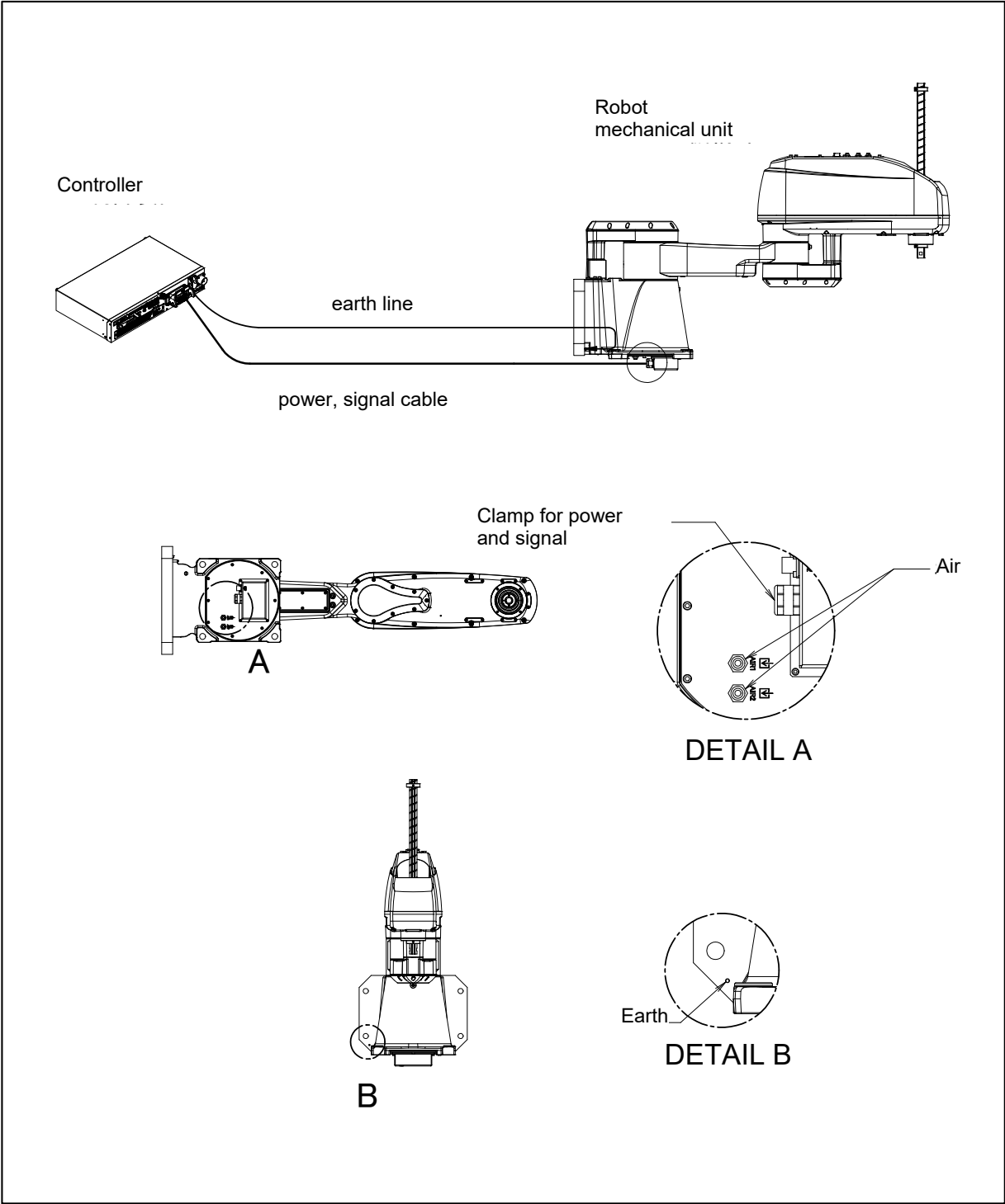
Fig. 2 (c) Cable connection (wall mount specification)
