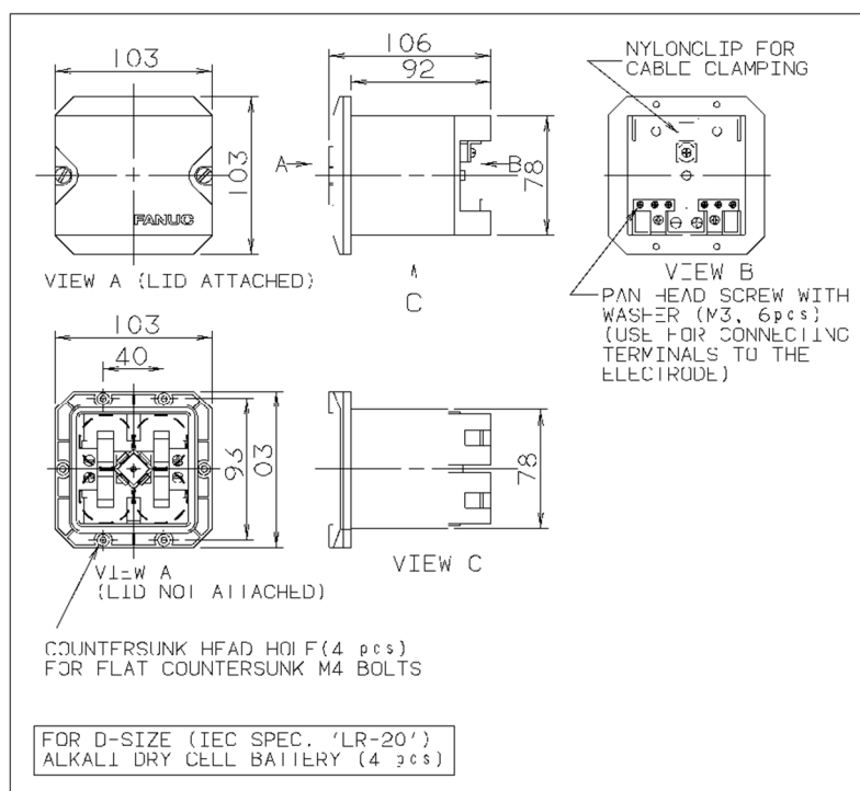
Fig. 7.3.1 (a) External dimensions of the battery box
