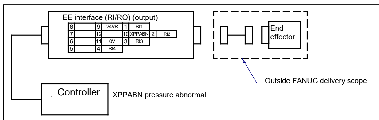
Fig. 5.2 (d) EE (RI/RO) interface (When A05B-1118-H202,H252,H302,H352 is specified)
