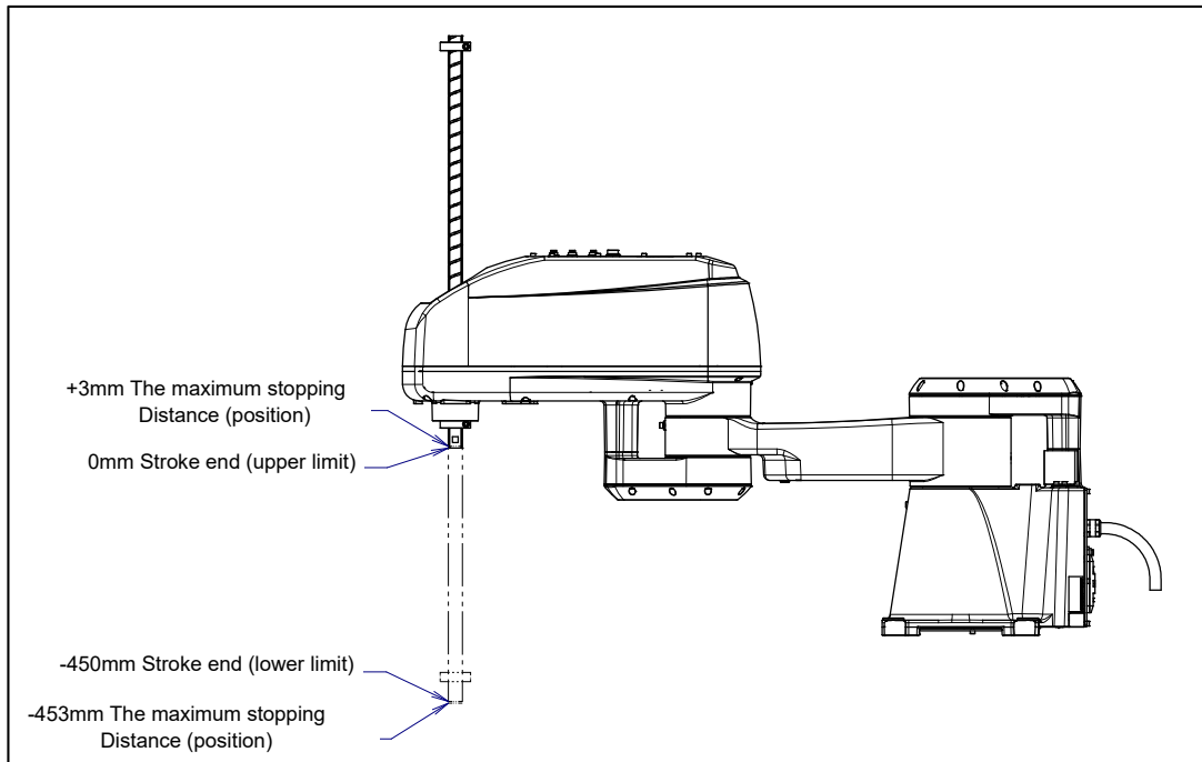
Fig. 3.3 (e) J3-axis motion limit (450mm stroke)
