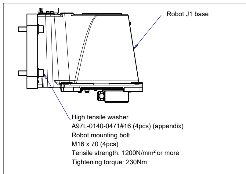
Fig. 1.2.1 (b) Actual Installation Example (wall mount)
