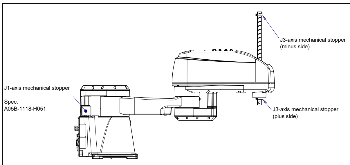
Fig. 3.3 (a) Position of mechanical stopper
