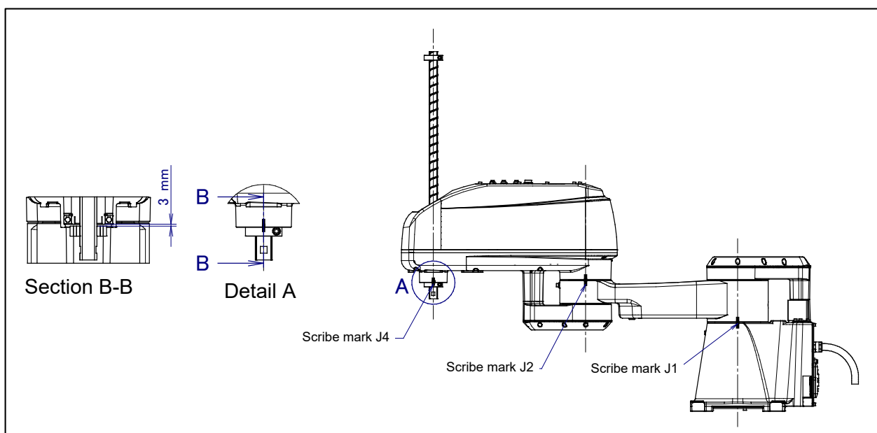
Fig. 8.3 (a) Marking position
