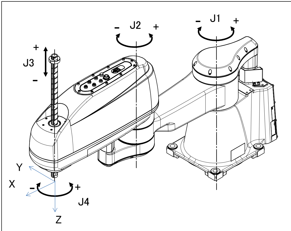
Fig. 3.1 (b) Each axis coordinates and mechanical interface coordinates
